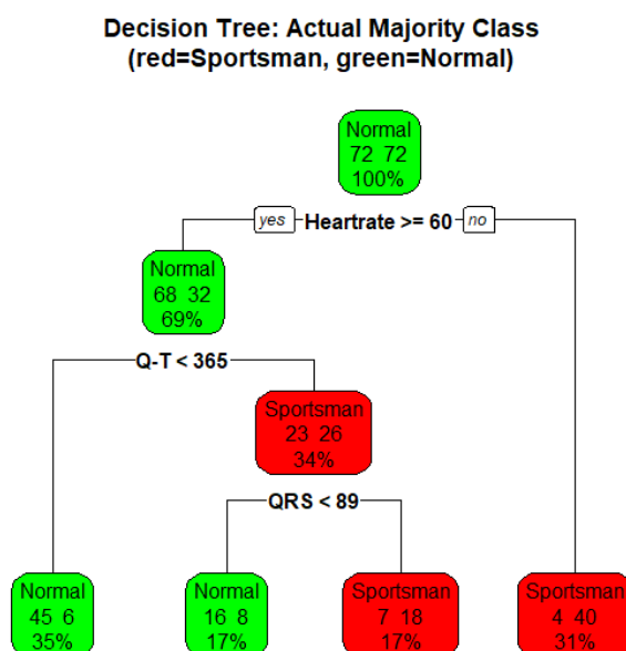
Fig. 1. Decision Tree for classifying Sportsmen from Normal
